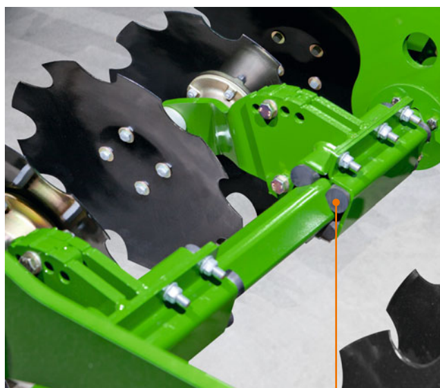
Rubber suspension elements
